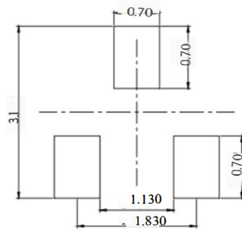
DIMENSIONS:MILLIMETERS
