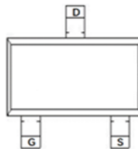
Pin Assignment
